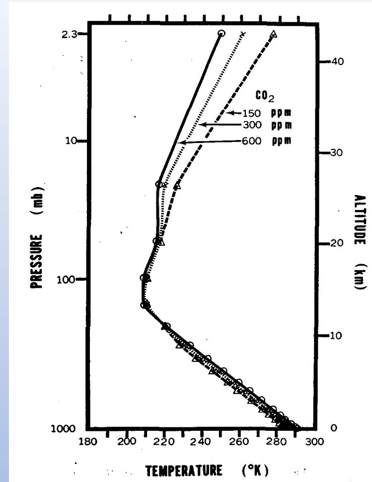
A figure from the memorial work of Manabe and Wetherald (1967), on the nature of the radiative-convective equilibrium and the climate response due to changes in carbon dioxide concentrations.
