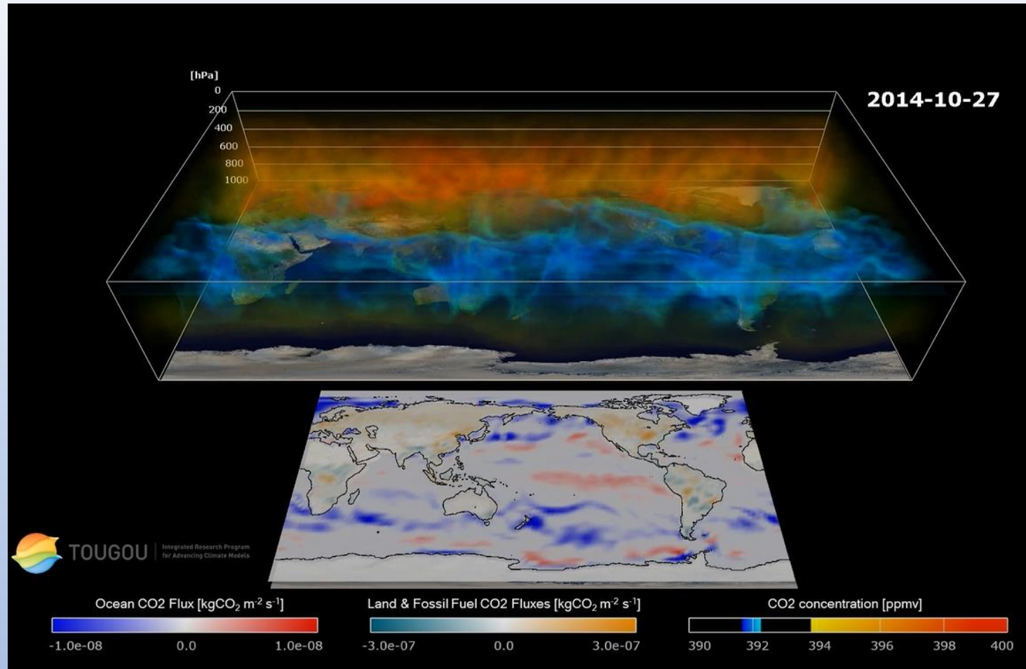
Three-dimensional distribution of atmospheric CO 2 (upper) and a map of carbon source and sink (lower), both reproduced by an Earth system model MIROC-ES2L
