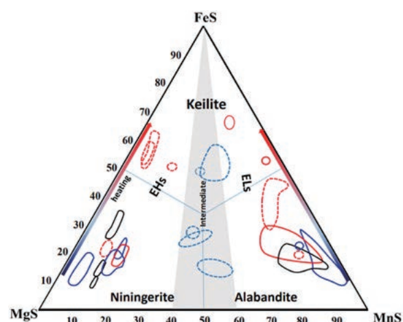
The compositions of (Mg,Mn,Fe)S, a key indicator for condensation and metamorphism of enstatite chondrites
