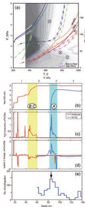
Fig. 1 (a) P–T paths of the subducting crust for six subduction zones. Shading shows maximum H_2O contents in wt%. (b) Accumulated dehydration-derived H_2O content in wt%, (c) rate of H_2O production and (d) total system (solid + H_2O ) volume for Hokkaido (blue lines) as a representative cold slab, and for Kii (red lines) as a representative warm slab. In (c), Kii is scaled by a factor of 10. (e) Frequency of upper-plane earthquakes beneath central Hokkaido as a function of depth.
