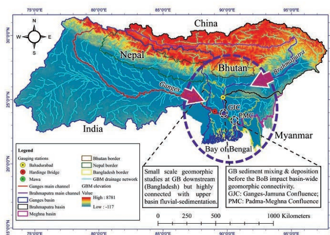
An overview of geomorphic connectivity in the Ganges-Brahmaputra Basin with a focus on Bangladesh in the downstream domain
