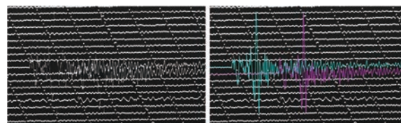
Fig.2 Part of long-period north-south motion recorded at COL station (College, Alaska) on December 19, 1966. (Left) The section of the scanned microfiche image. (Right) Same image with digitized traces for two of the lines shown in cyan and magenta.
