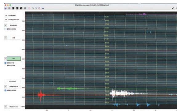
Fig.1 Screenshot of DigitSeis version 1.6 \beta (with display in Japanese) showing the short-period vertical recording from Tucson, Arizona between July 15 and 16, 1945. Digitized traces in colour have been overlain on top of the scanned seismogram image with yellow vertical bars indicating each minute (each hour is also labelled in yellow). The large arrivals in white are those associated with the Trinity nuclear test.
