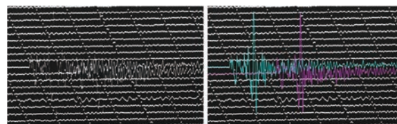
Fig.2 Part of long-period north-south motion recorded at COL station (College, Alaska) on December 19, 1966. (Left) The section of the scanned microfiche image. (Right) Same image with digitized traces for two of the lines shown in cyan and magenta.
