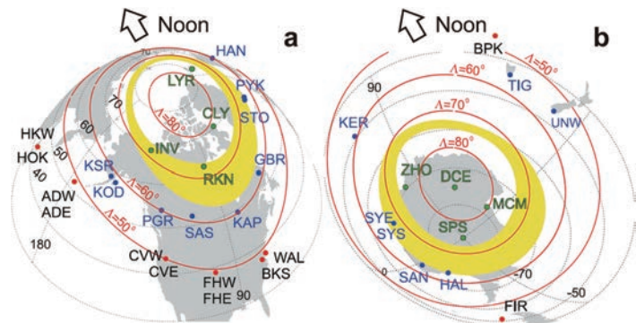
Schematic plots showing the a Northern and b Southern Hemisphere SuperDARN radar locations with respect to the auroral oval. The model auroral oval (yellow) for moderately disturbed conditions is plotted with the SuperDARN radar locations identified in green type and green closed circles (polar cap latitudes), blue type and blue closed circles (auroral latitudes), and black type and red closed circles (mid-latitude radars).
