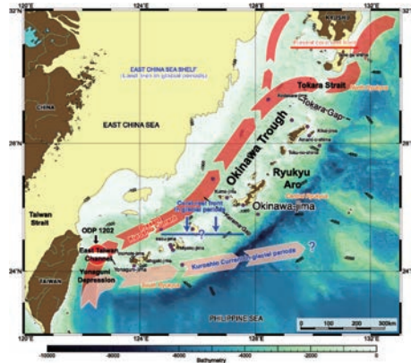
Figure 1: The southern path of the Kuroshio Current showing the inferred extent of the Ryukyu Reefs in glacial and interglacial periods (adapted from Iryu et al. [2006])
