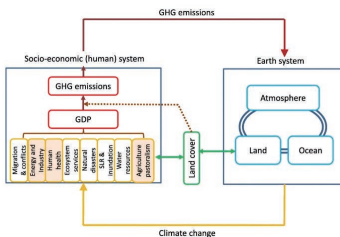
Conceptual diagram of the Earth-human (socio-economic) system interaction.
