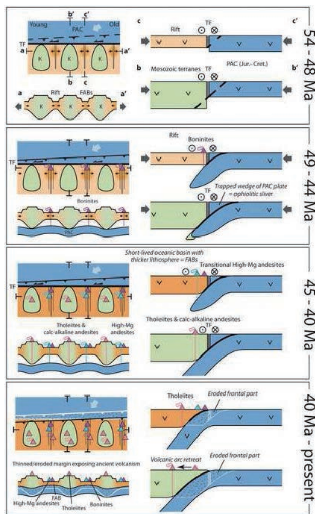
Schematic tectono-magmatic model of IBM subduction initiation and early evolution. Special emphasis has been done on the geodynamic context of various magma 1 eruptions. The white lines in stage “40 Ma - present” represent the former positions of plate boundaries or the base of the upper plate in stage “45-40 Ma”.
