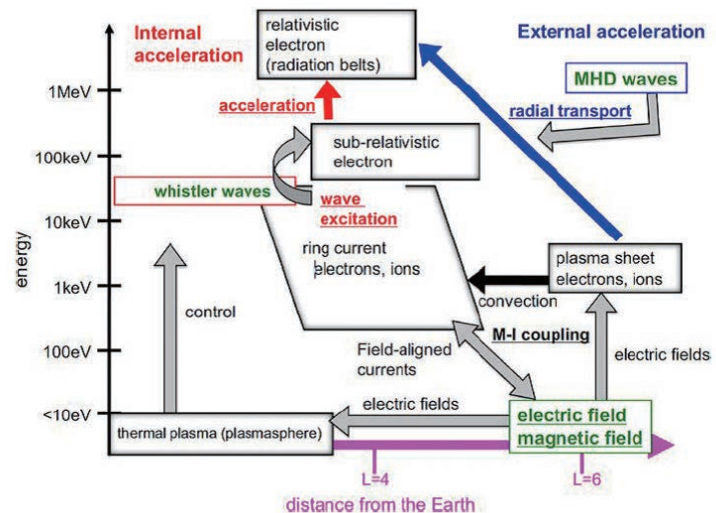
Diagram illustrating the interconnectedness and cross-energy coupling between particles, waves, and underlying physical processes.
