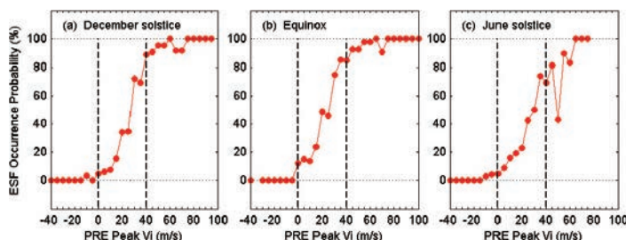
The dependence of the plasma bubble occurrence probability on the vertical ion drift at the PRE peak measured by C/NOFS during May 2008–June 2013 for different seasons.
