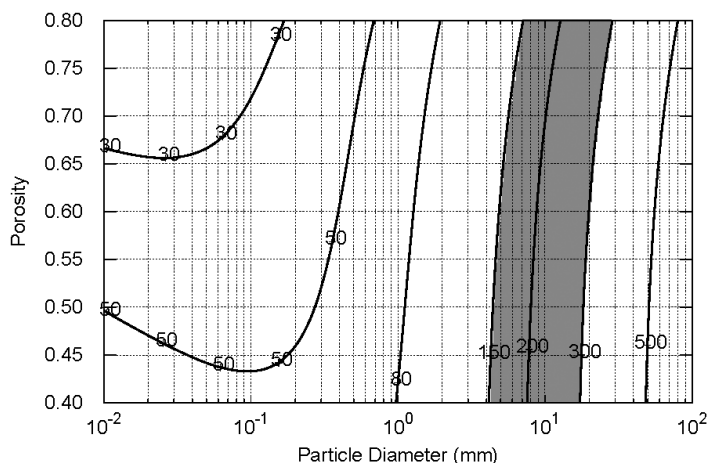
Contour plot of thermal inertia (in units of \text{J m}^{-2} \text{s}^{-1/2} \text{K}^{-1} ) as a function of typical particle diameter and porosity (see text for the regolith parameters assumed in the calculation). The gray-filled region indicates the thermal inertia range estimated for Ryugu by ground-based observations (Müller et al. 2017). From this figure, we can estimate a typical particle size for the Ryugu regolith.
